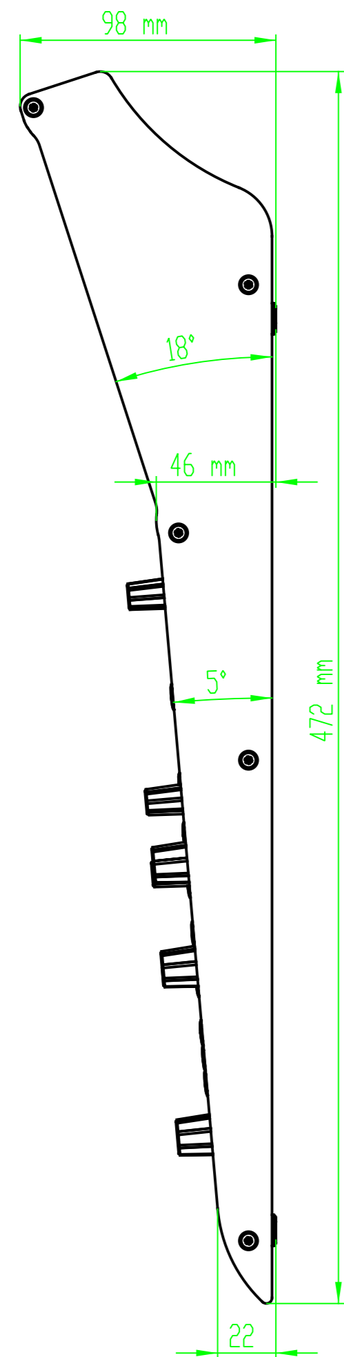
Side view
