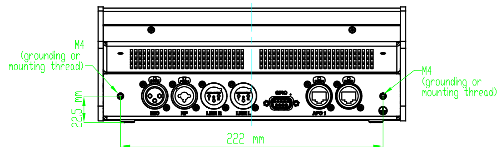
Rear view
