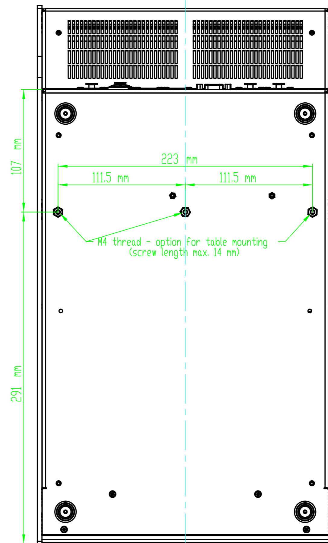
Bottom view
