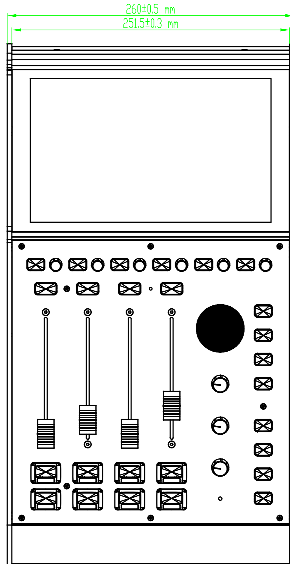
Top view
