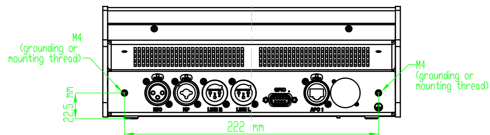
Rear view
