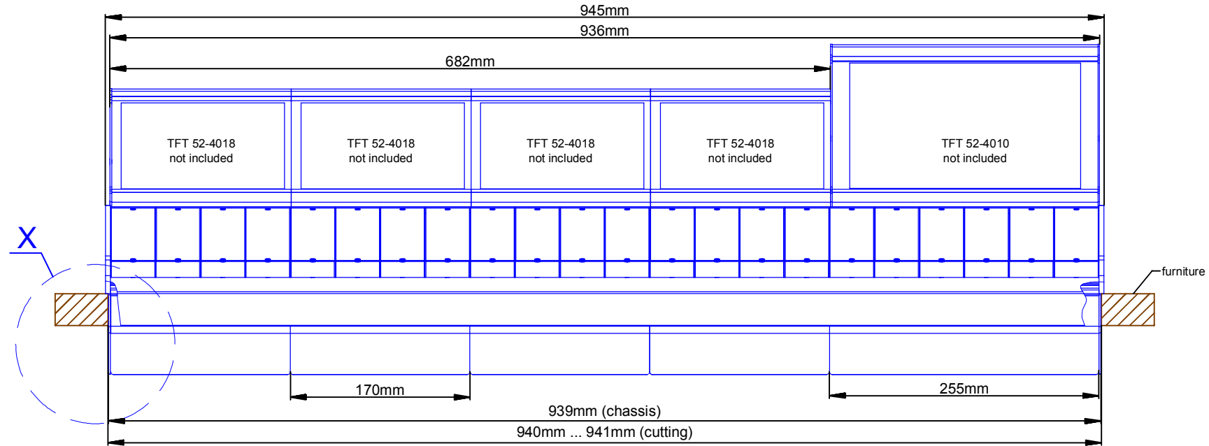
cut A - A
