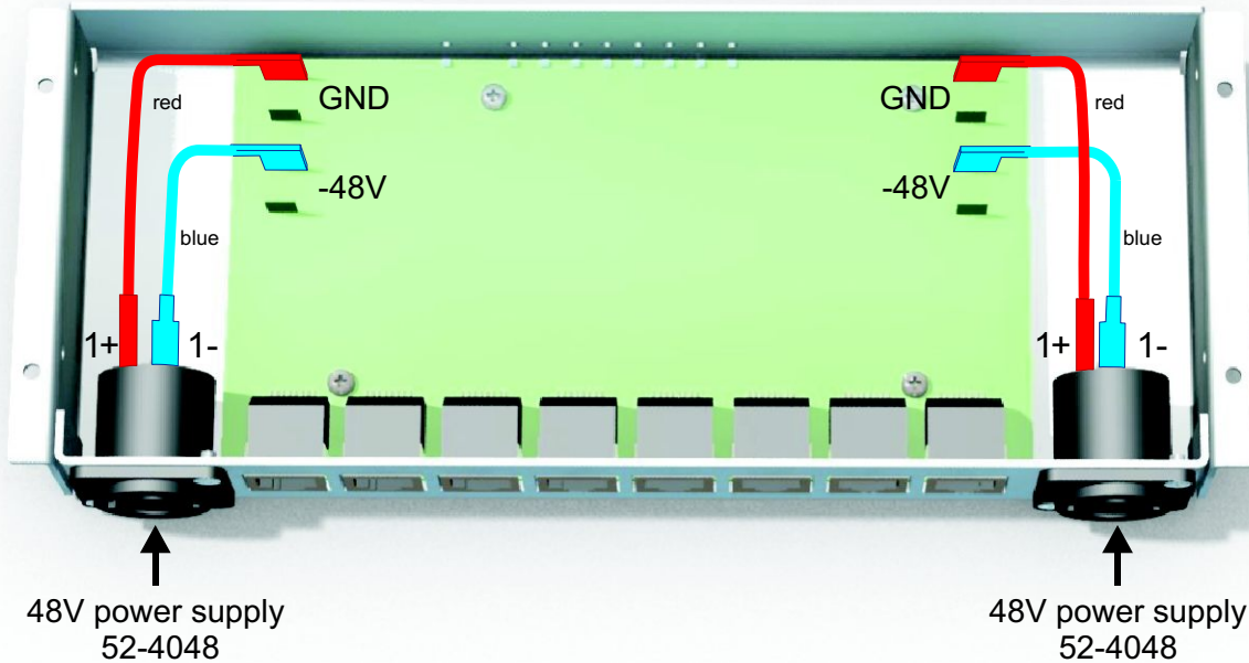
redundant wiring - factory default
