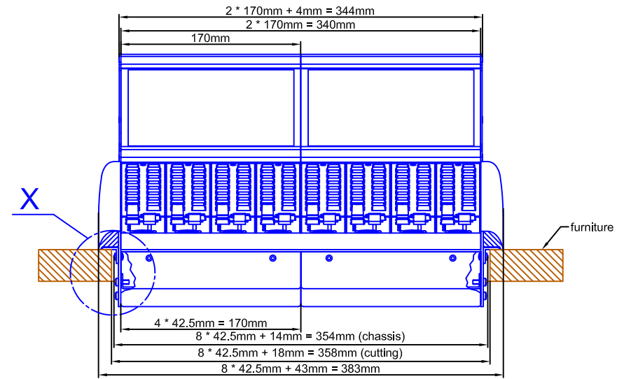
cut A - A
