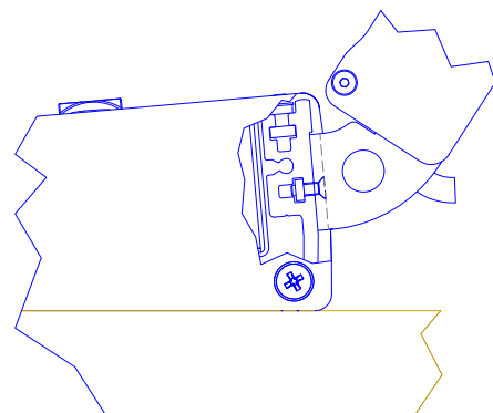
view X, scale 1:2
