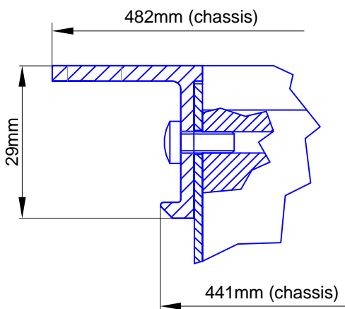
view X, scale 1:1
