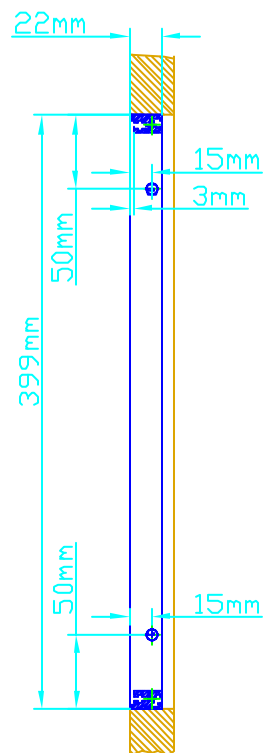
Cut B-B
