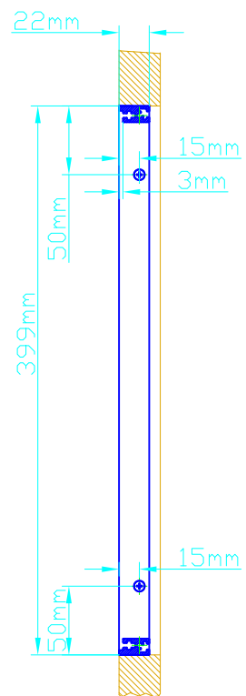
cut B-B
