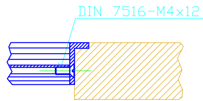
cut B-B
