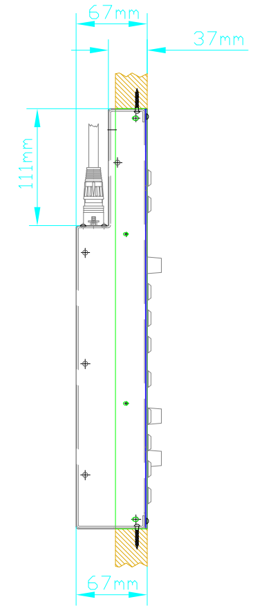
View Y (scale 1:1) (version 2)
