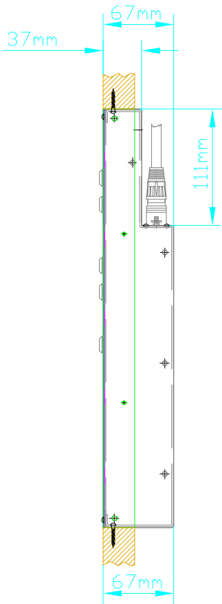
View X (scale 1:1) (version 1)
