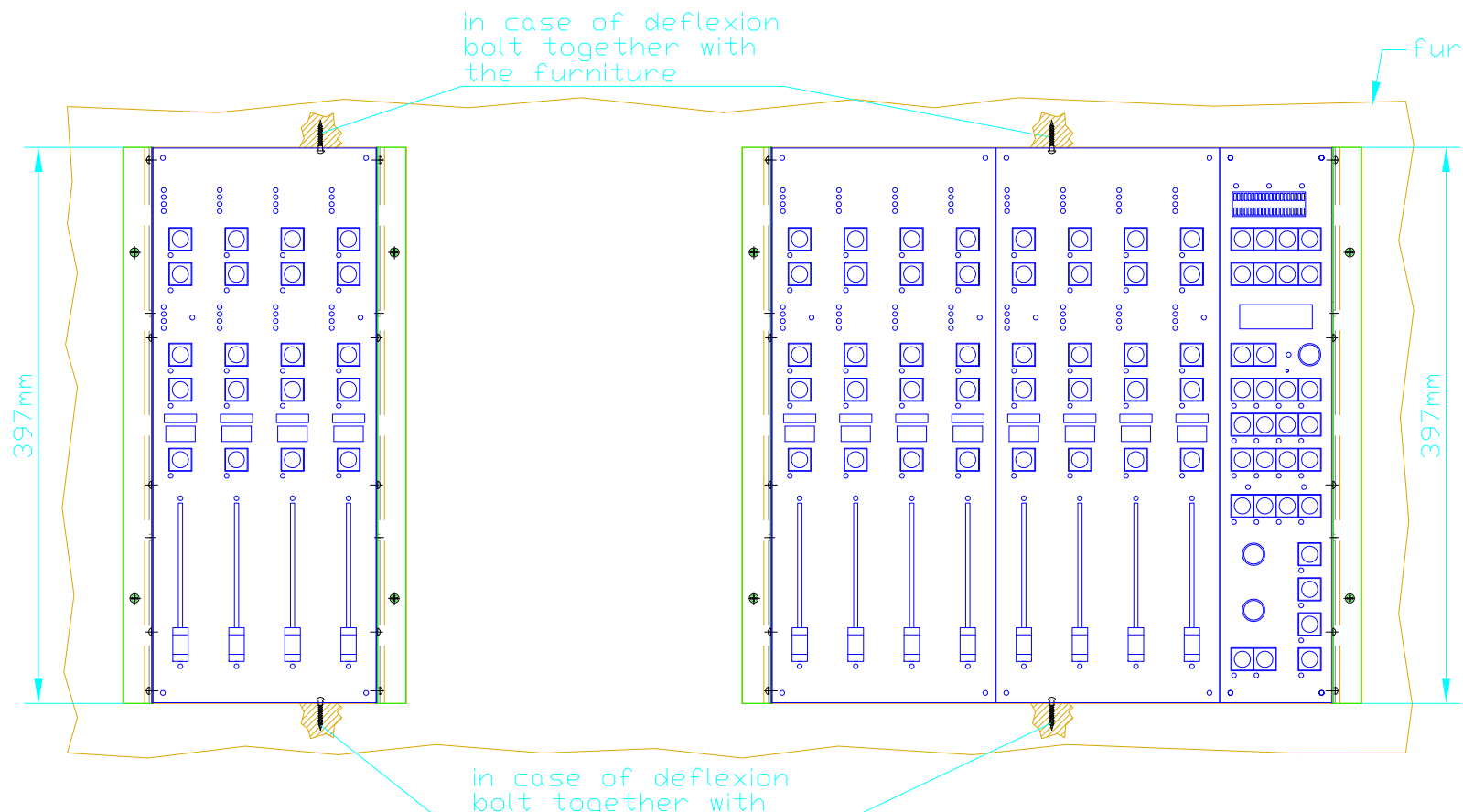
View X (scale 1:1) (version 2)
